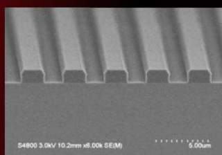
L/S 2 \mu\text{m}
