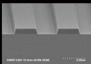
L/S 5 \mu\text{m}
